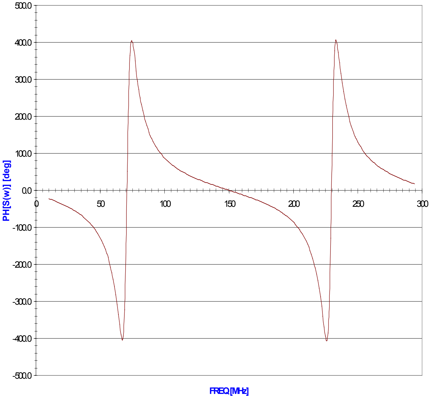
CHANNEL XFER FUNCTION PHASE (Beta=0.99; Delta(Phi)=2.8; Tau=6.3ns)
