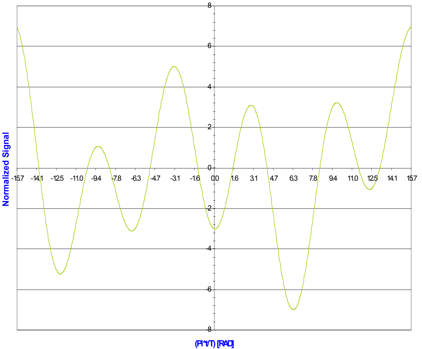
Typical Multi-Level Raised-Cosine 64QAM
