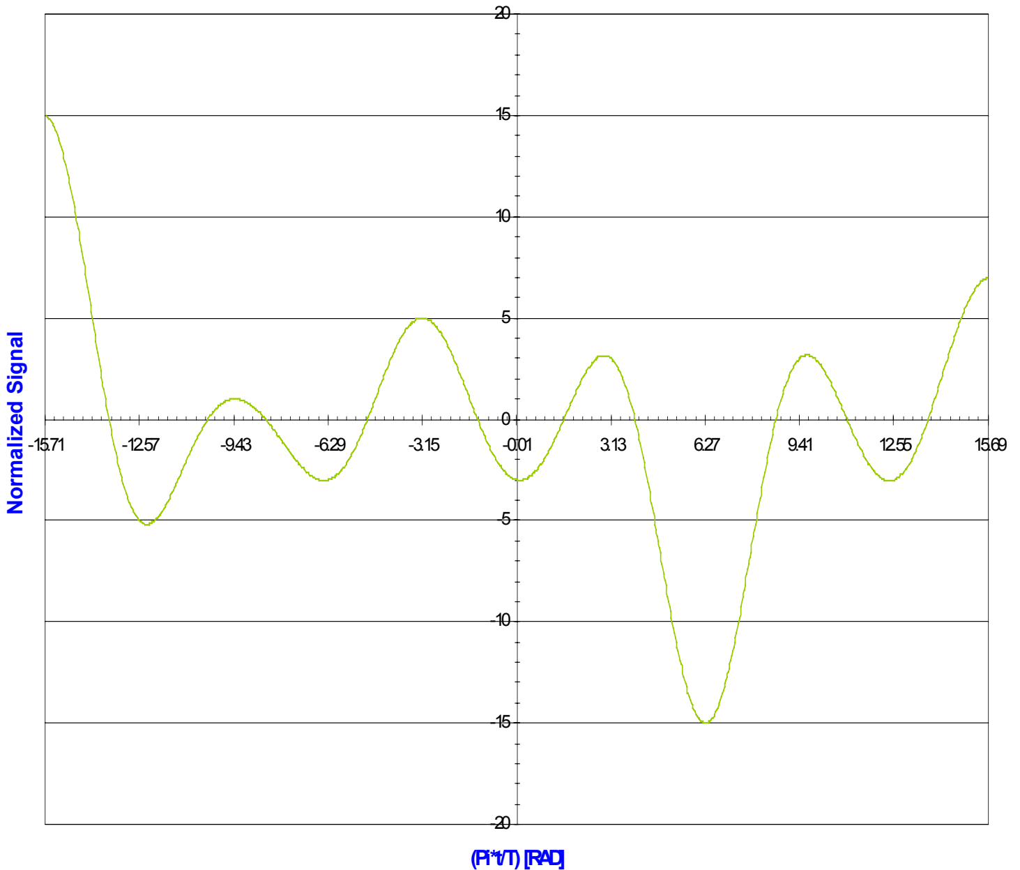
Typical Multi-Level Raised-Cosine 256QAM
