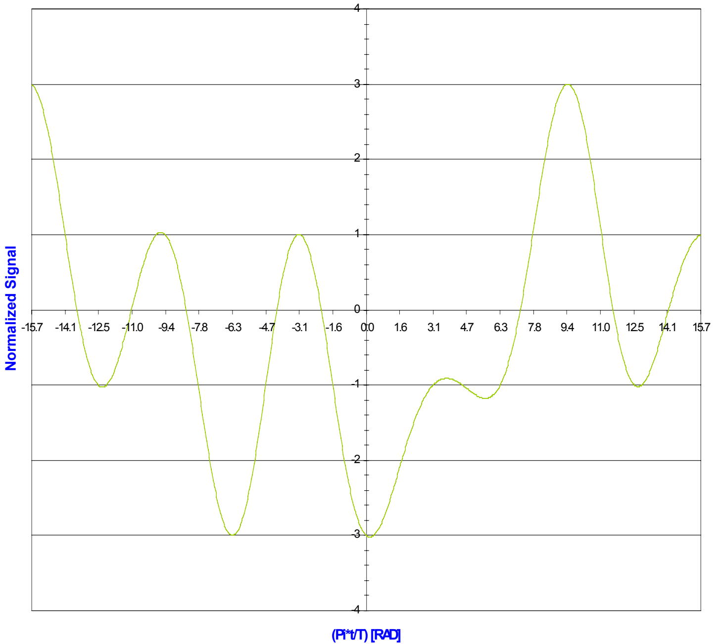
Typical Multi-Level Raised-Cosine 16QAM
